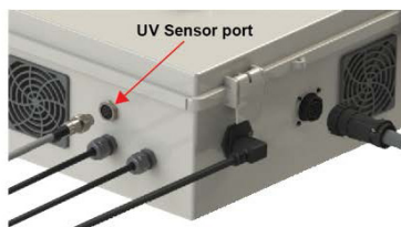
Figure 7. Sensor Connection
